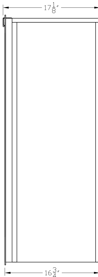
SIDE VIEW
